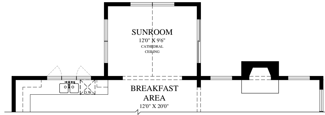
PARTIAL FIRST FLOOR PLAN AT OPTIONAL SUNROOM
