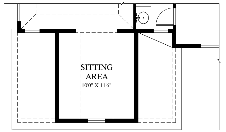
PARTIAL SECOND FLOOR PLAN AT OPTIONAL SITTING AREA
