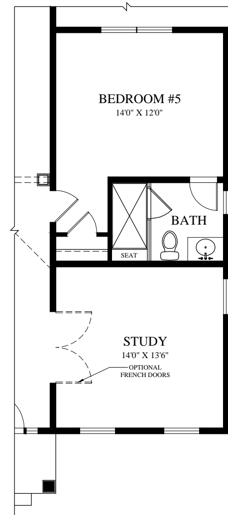
PARTIAL FIRST FLOOR PLAN AT OPTIONAL BEDROOM #5
