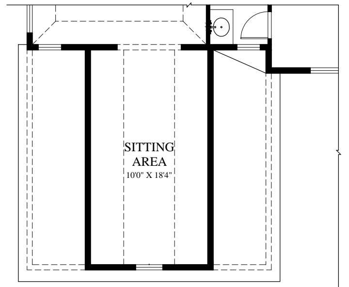
PARTIAL SECOND FLOOR PLAN AT OPTIONAL EXTENDED SITTING AREA
