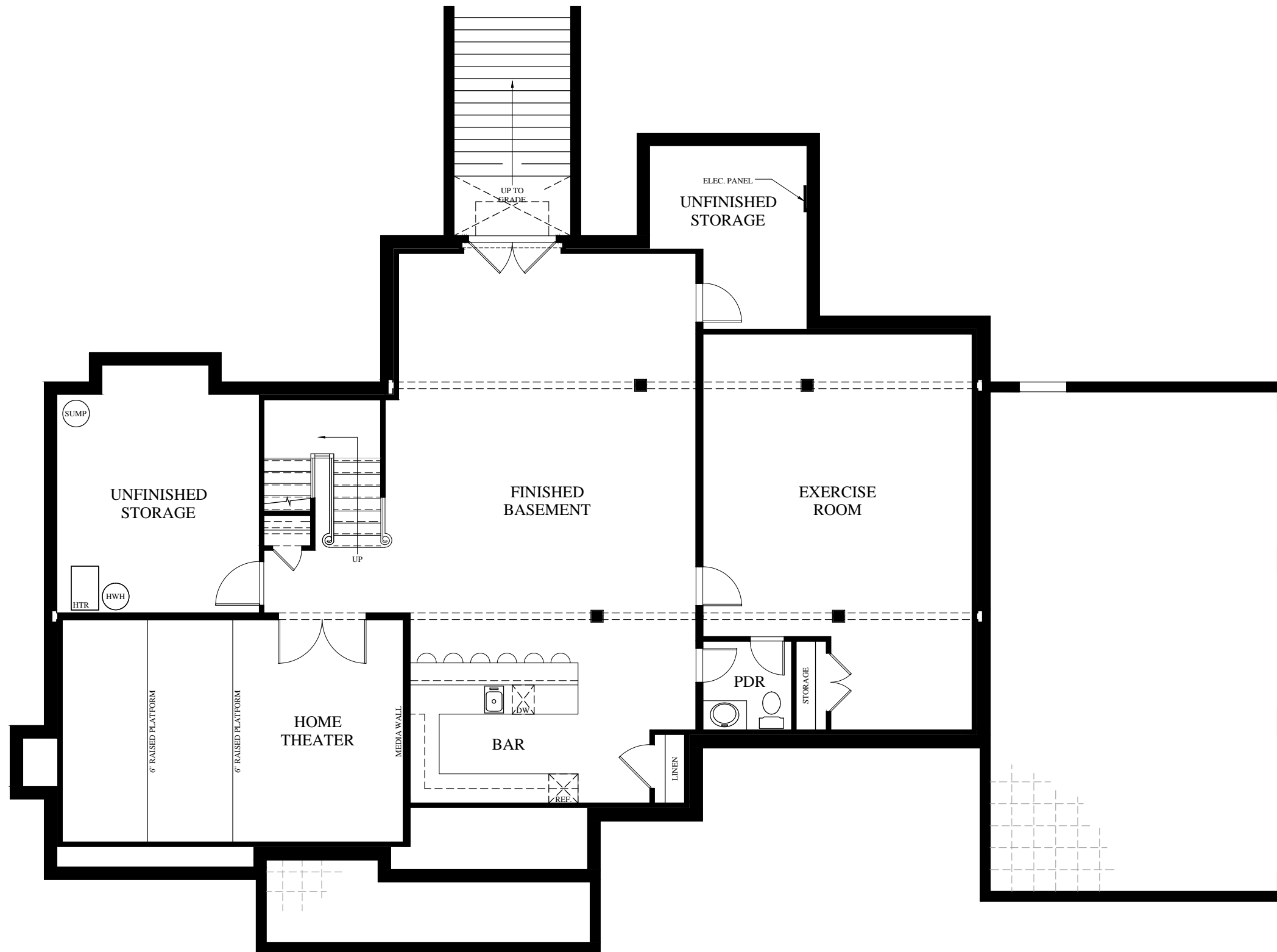
OPTIONAL FINISHED BASEMENT PLAN 9'-0" CEILING HEIGHT
