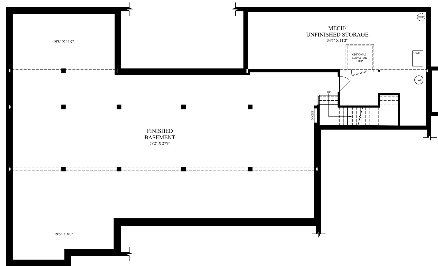
OPTIONAL FINISHED BASEMENT
